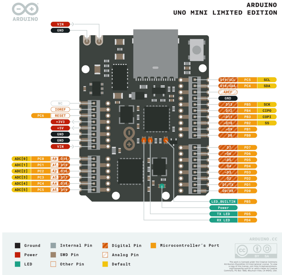
Pinout
