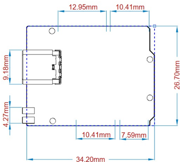
Board outline
