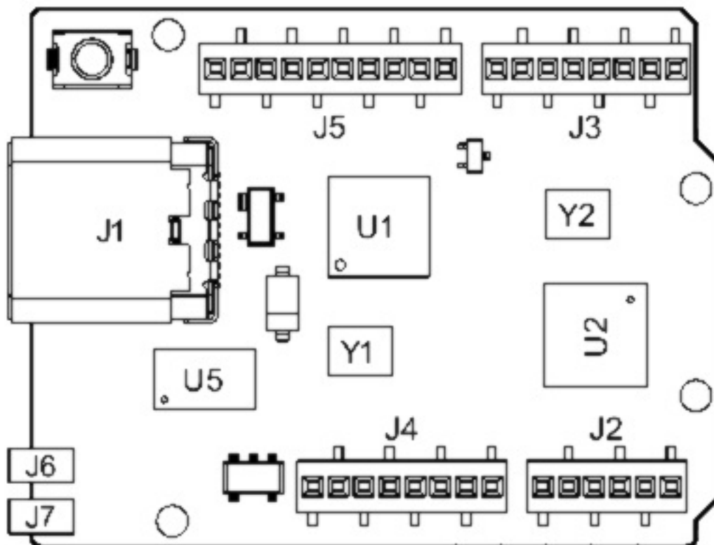
Board topology, Top
